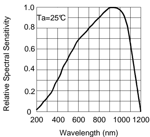
FIG.3 SPECTRAL SENSITIVITY
