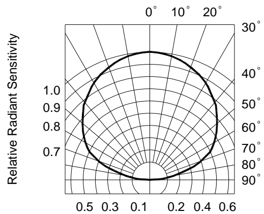
FIG.4 SENSITIVITY DIAGRAM
